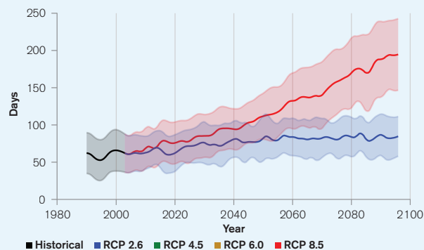
FIGURE 11. Increase in the annual average number of hot days (>35°C) in Cambodia under two emissions pathways. RCP2.6 (blue) and RCP8.5 (red). 63
