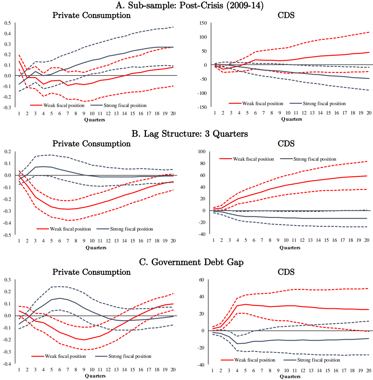
Figure 5: Ricardian and Interest Rate Channels: Impulses Responses
