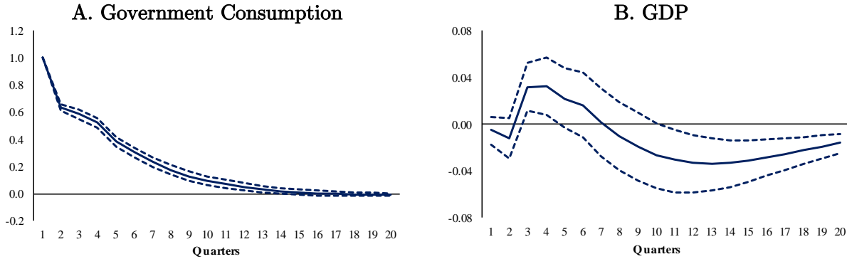
Figure A.2: Unconditional Impulse Responses
